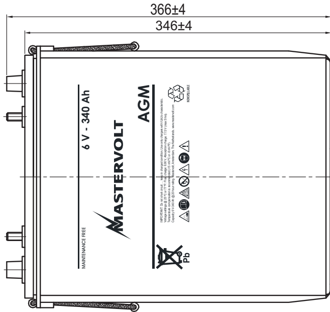
Side view AGM - 6V 340Ah
