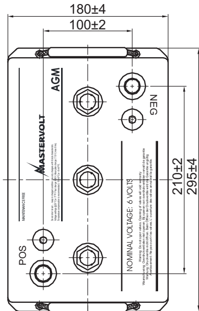
Top view (all models)
